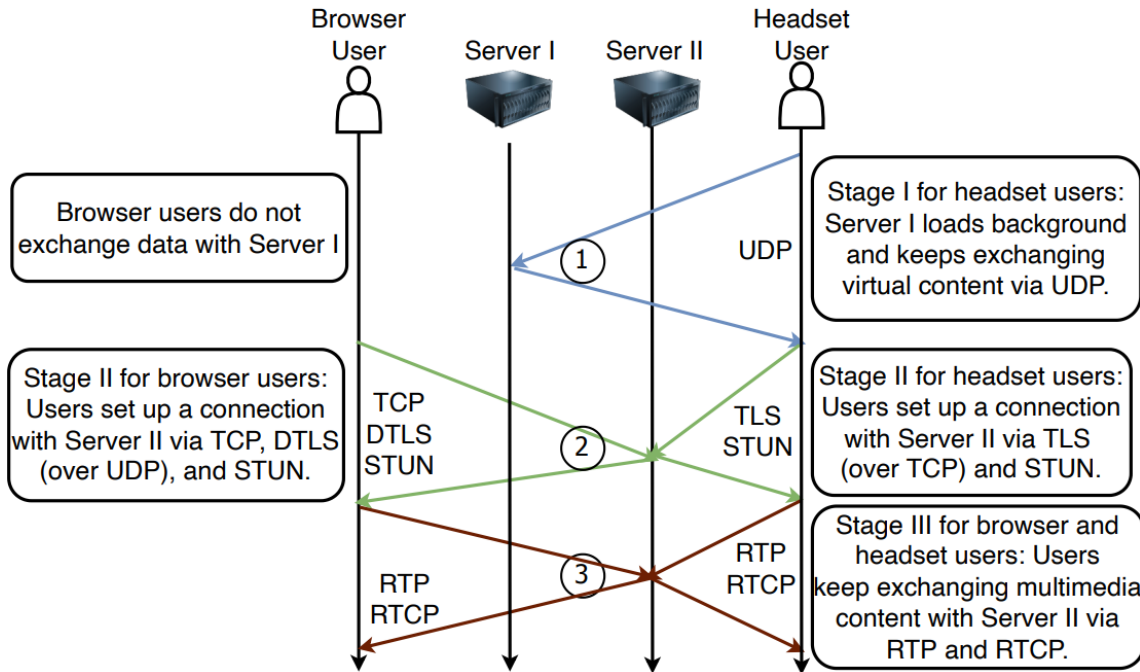
Figure 1: The process of establishing connections and exchanging data between the clients and the servers.
